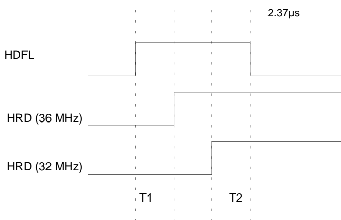
Fig.9 Time relation between HDFL and HRD (32MHz and 36MHz)
